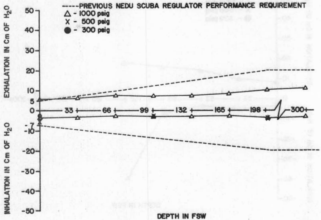
Figure 12B-2. Tekna T-2100B Breathing resistance vs. depth at 40 RMV
