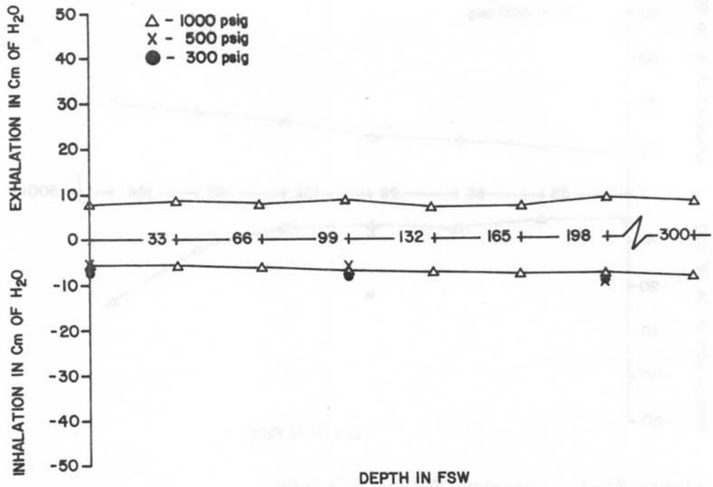
Figure 8A-1. Sherwood Selpac SRB-2000 Breathing resistance vs. depth at 22.5 RMV
