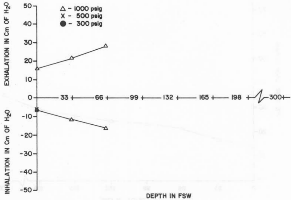
Figure 2C-5. Dacor Pacer 300 Breathing resistance vs. depth at 90 RMV
