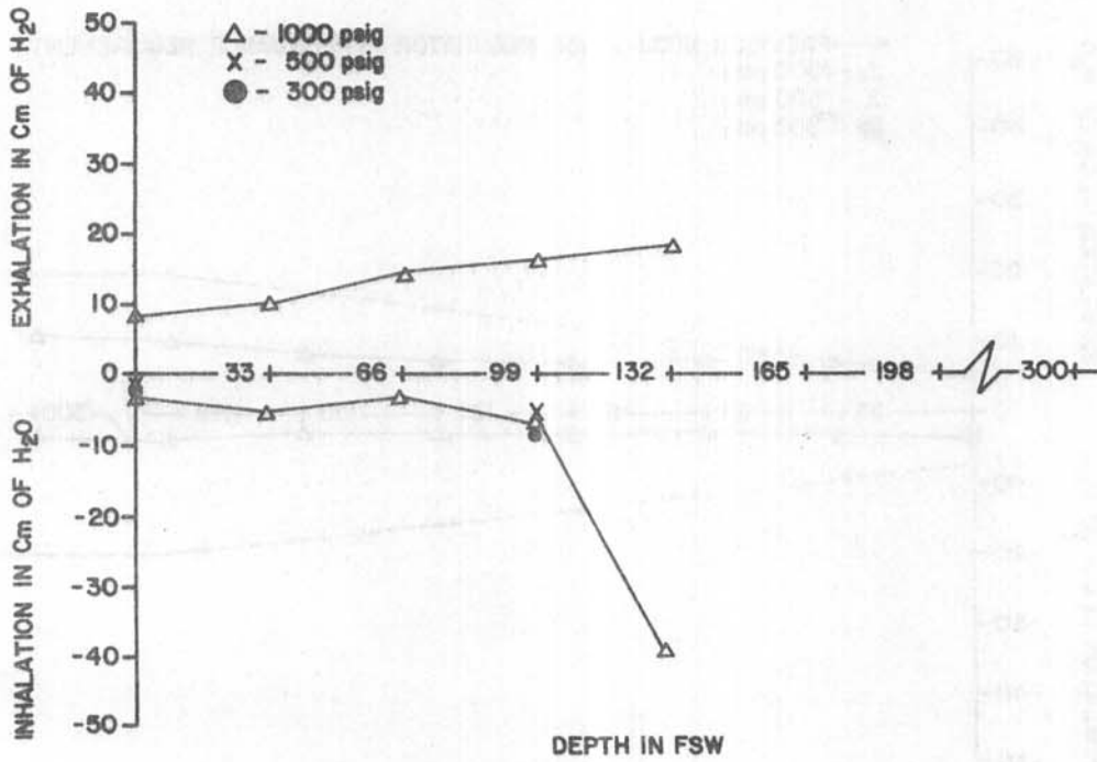
Figure 12B-4. Tekna T-2100B Breathing resistance vs. depth at 75 RMV
