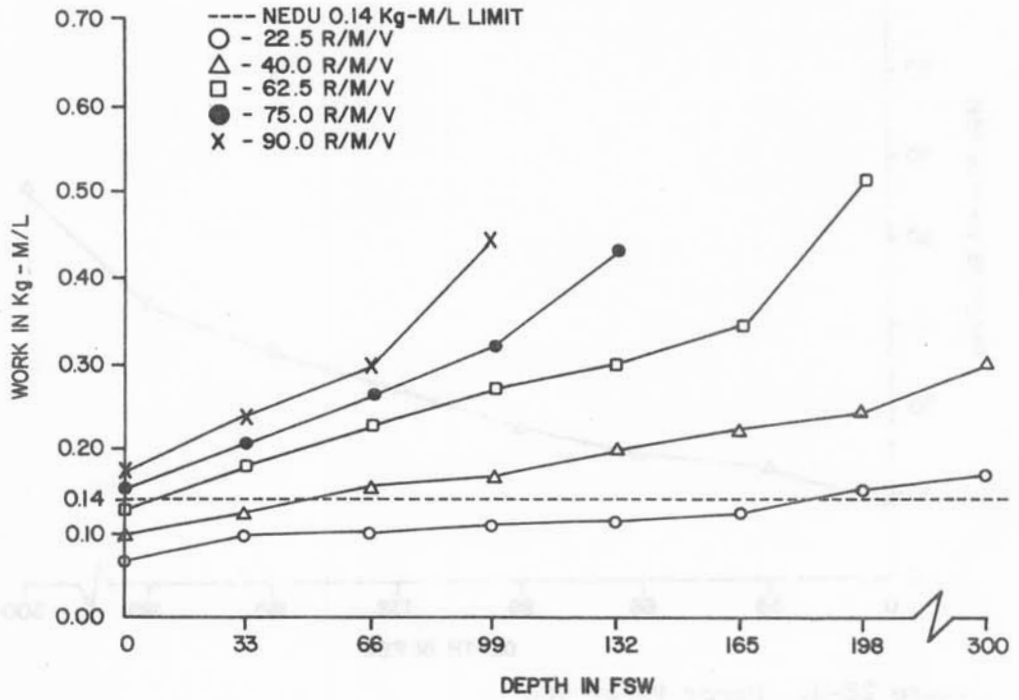
Figure 2E-6. Dacor Pacer 900 Breathing work vs. depth at 1000 psig supply pressure
