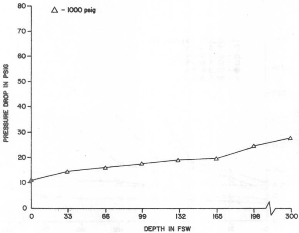
Figure 11C-8. Swimmaster MR12-II First stage pressure drop vs. depth at 40 RMV
