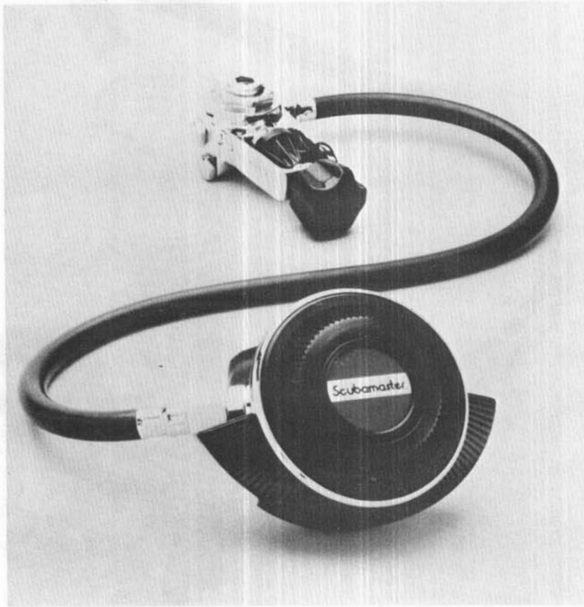
Scubamaster Model 7687
