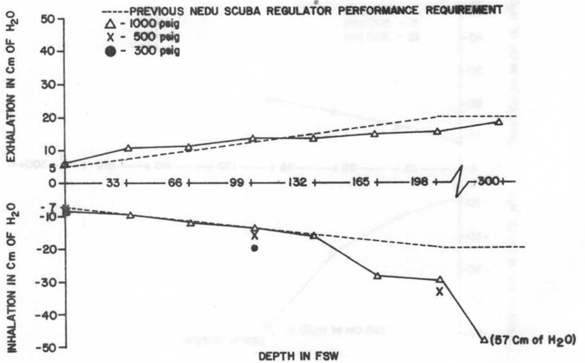
Figure 9E-2. Sportsways Model 1390 Breathing resistance vs. depth at 40 RMV
