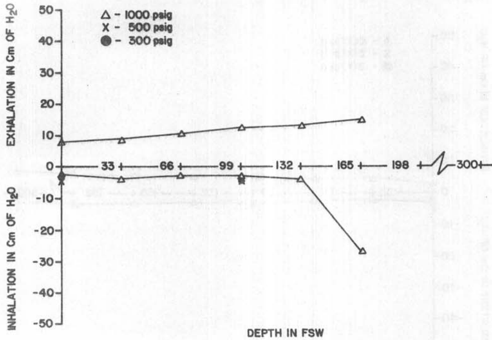
Figure 12B-3. Tekna T-2100B Breathing resistance vs. depth at 62.5 RMV
