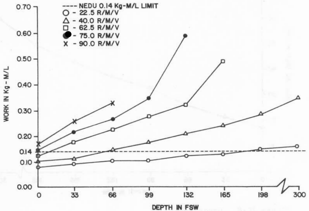
Figure 2C-6. Dacor Pacer 300 Breathing work vs. depth at 1000 psig supply pressure
