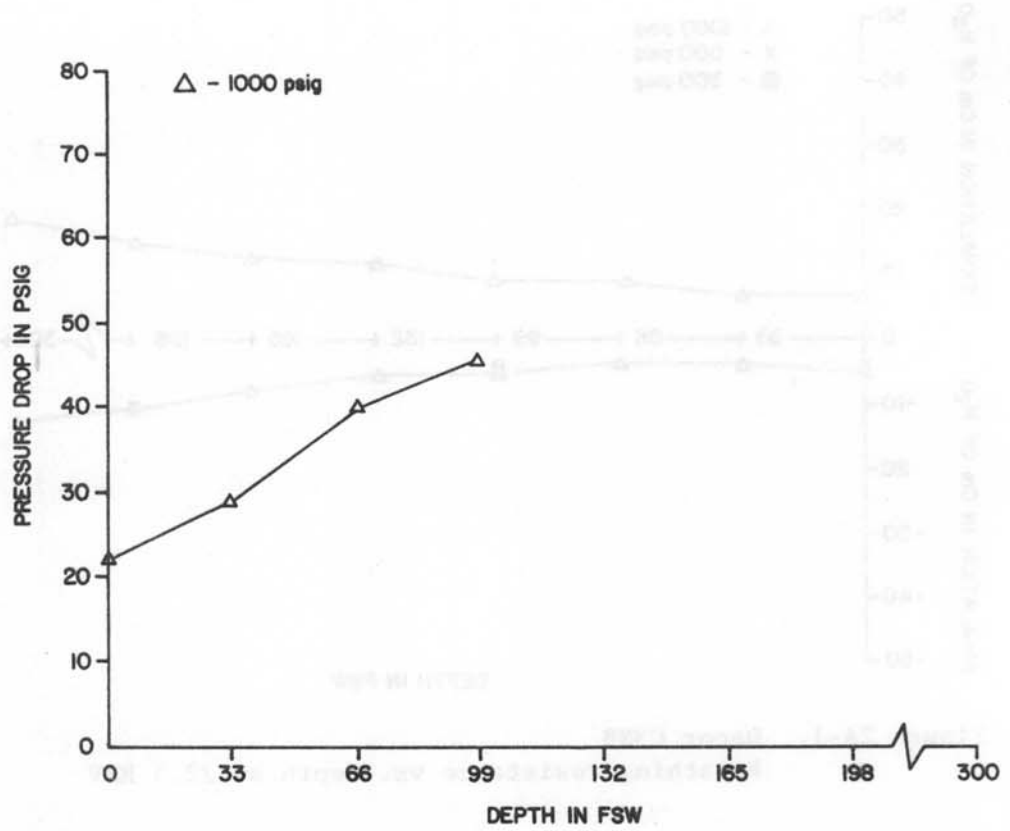
Figure 1A-11. AGA Divator 324/U.S.D. Conshelf XIV First stage pressure drop vs. depth at 90 RMV
