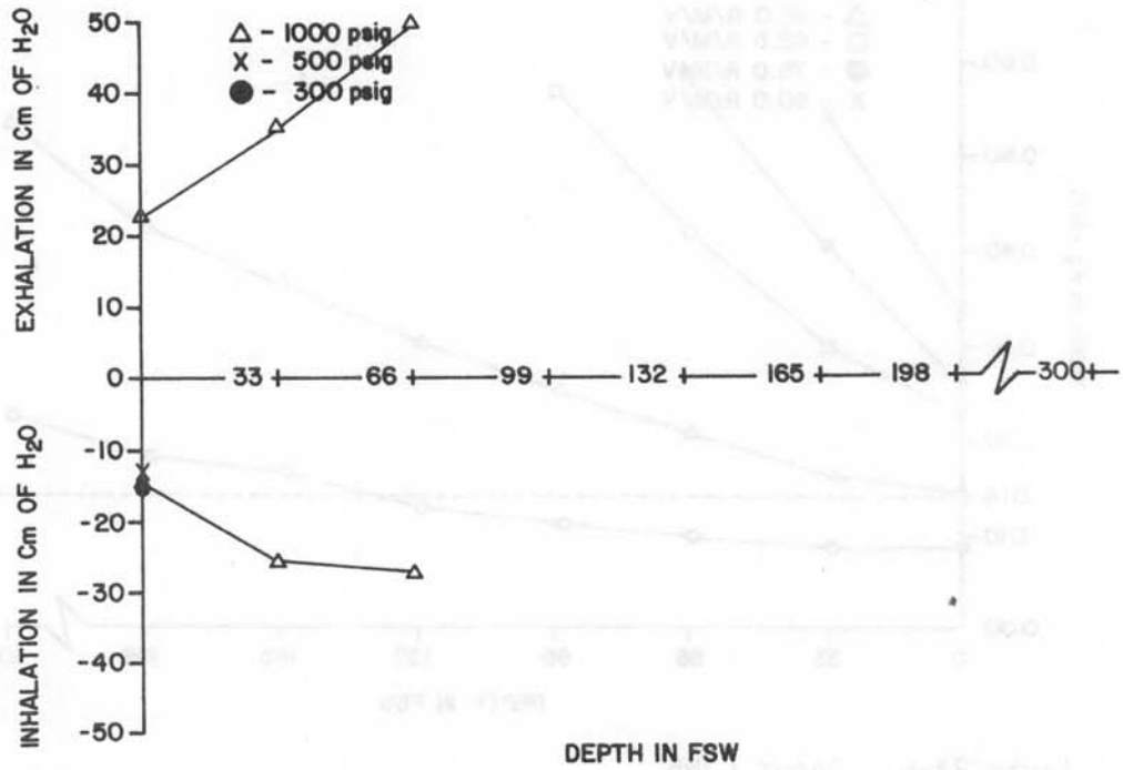
Figure 2A-4. Dacor C3NB Breathing resistance vs. depth at 75 RMV
