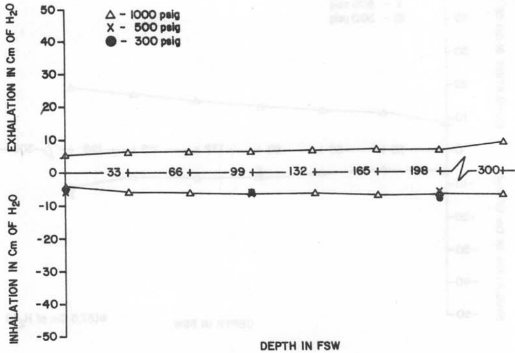
Figure 8B-1. Sherwood Selpac SRB-3100 Breathing resistance vs. depth at 22.5 RMV
