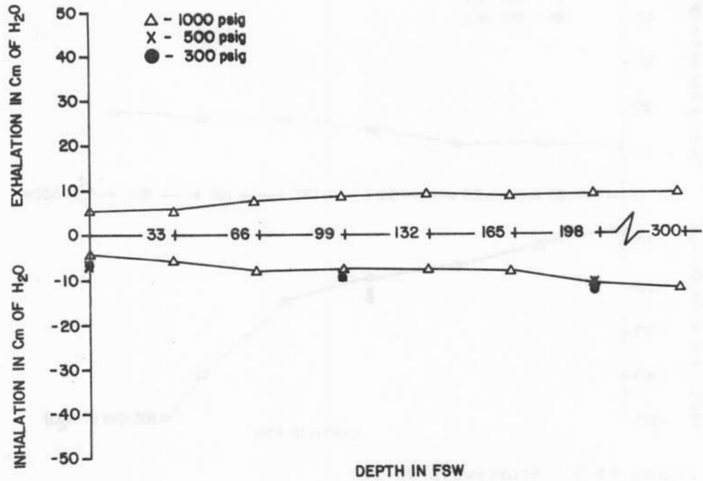
Figure 9A-1. Sportsways WL-200 Breathing resistance vs. depth at 22.5 RMV
