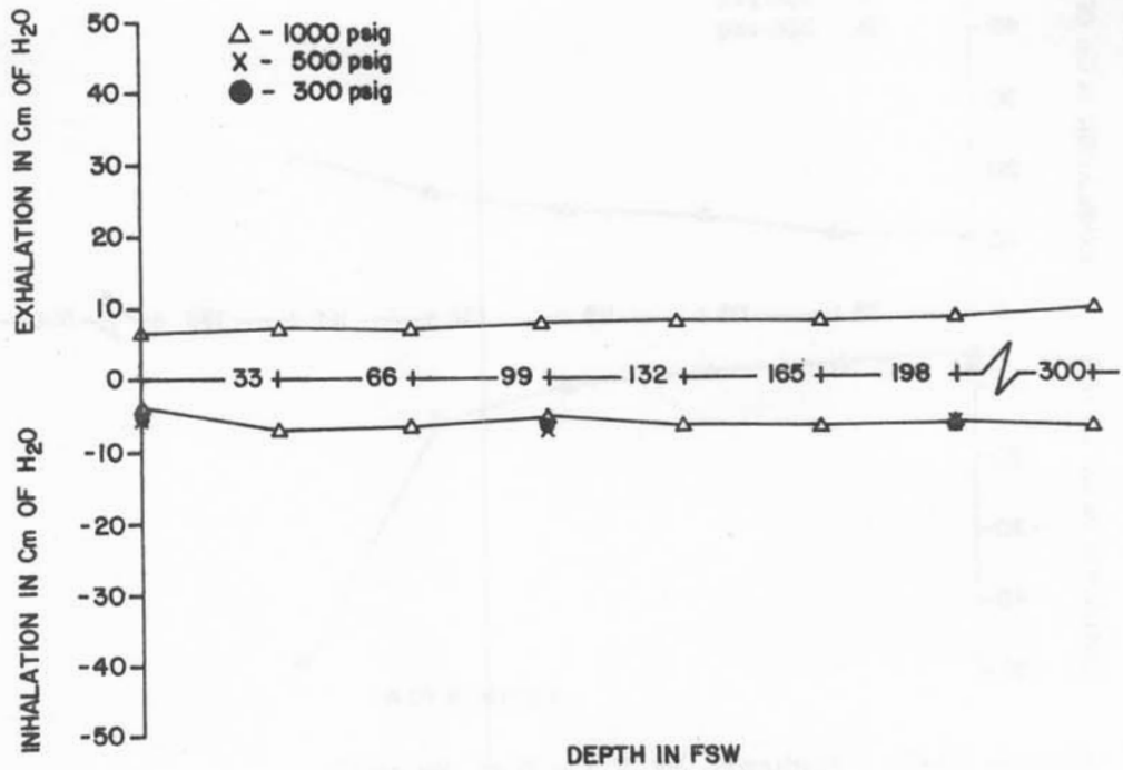
Figure 6A-1. Scubapro Mk V (4-Port Swivel) Breathing resistance vs. depth at 22.5 RMV
