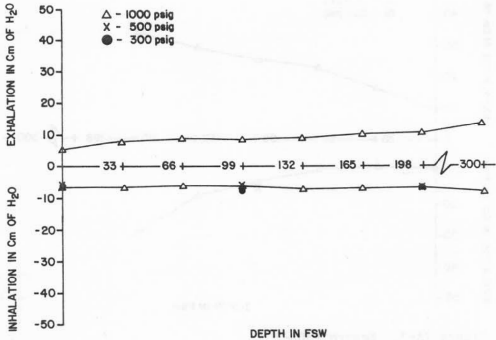
Figure 7A-1. Seapro FSDS-10 Breathing resistance vs. depth at 22.5 RMV
