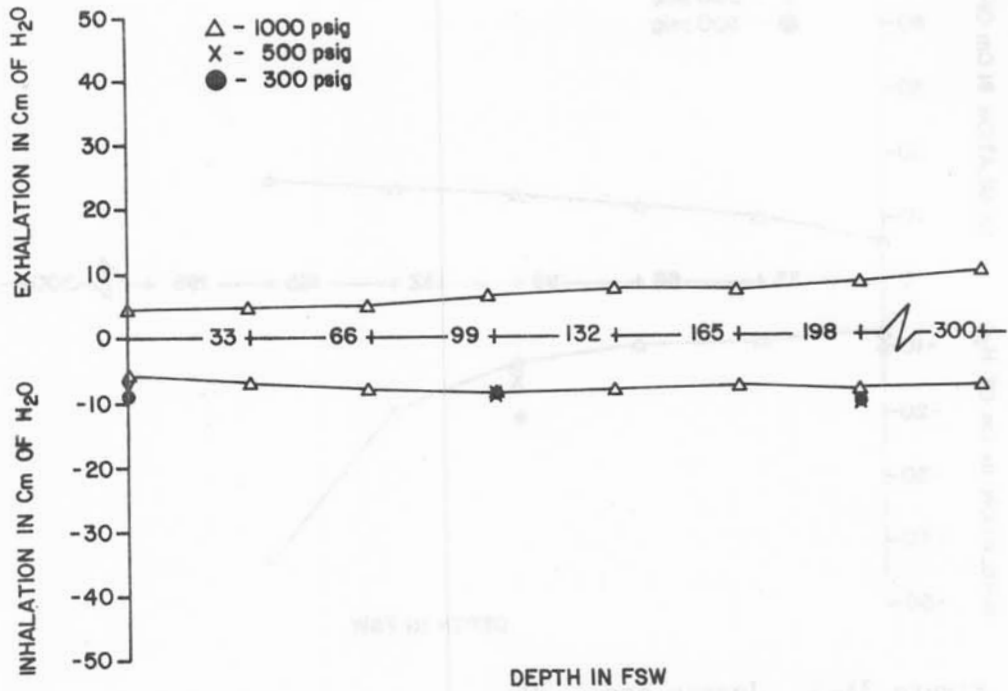
Figure 3A-1. Jepsen Model 200 Breathing resistance vs. depth at 22.5 RMV
