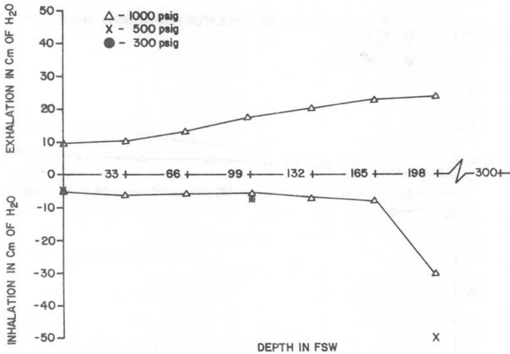
Figure 13C-4. U. S. Divers Conshelf XIV Breathing resistance vs. depth at 75 RMV
