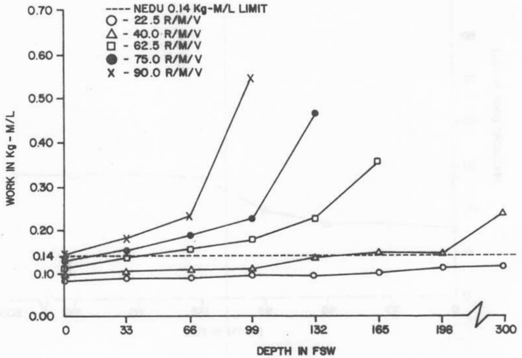
Figure 6A-6. Scubapro Mk V (4-Port Swivel) Breathing work vs. depth at 1000 psig supply pressure
