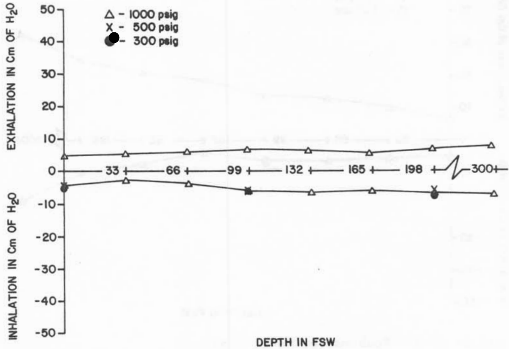
Figure 5A-1. Scubamaster Model 7687 Breathing resistance vs. depth at 22.5 RMV
