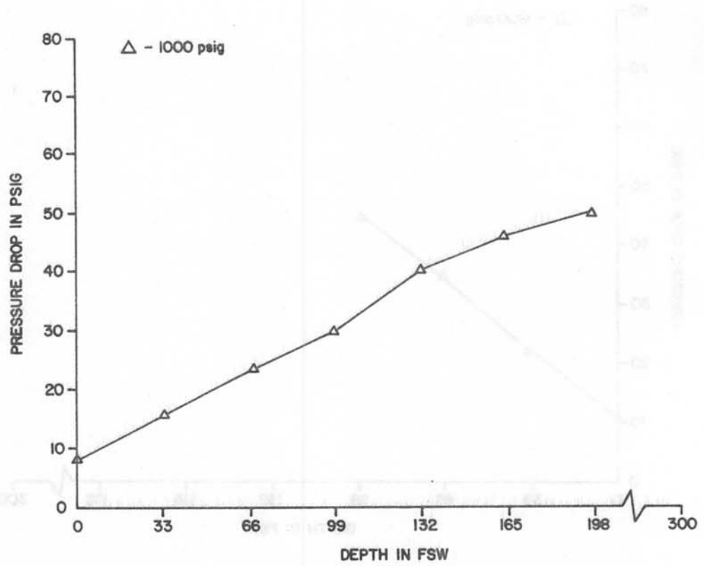
Figure 2E-9. Dacor Pacer 900 First stage pressure drop vs. depth at 62.5 RMV
