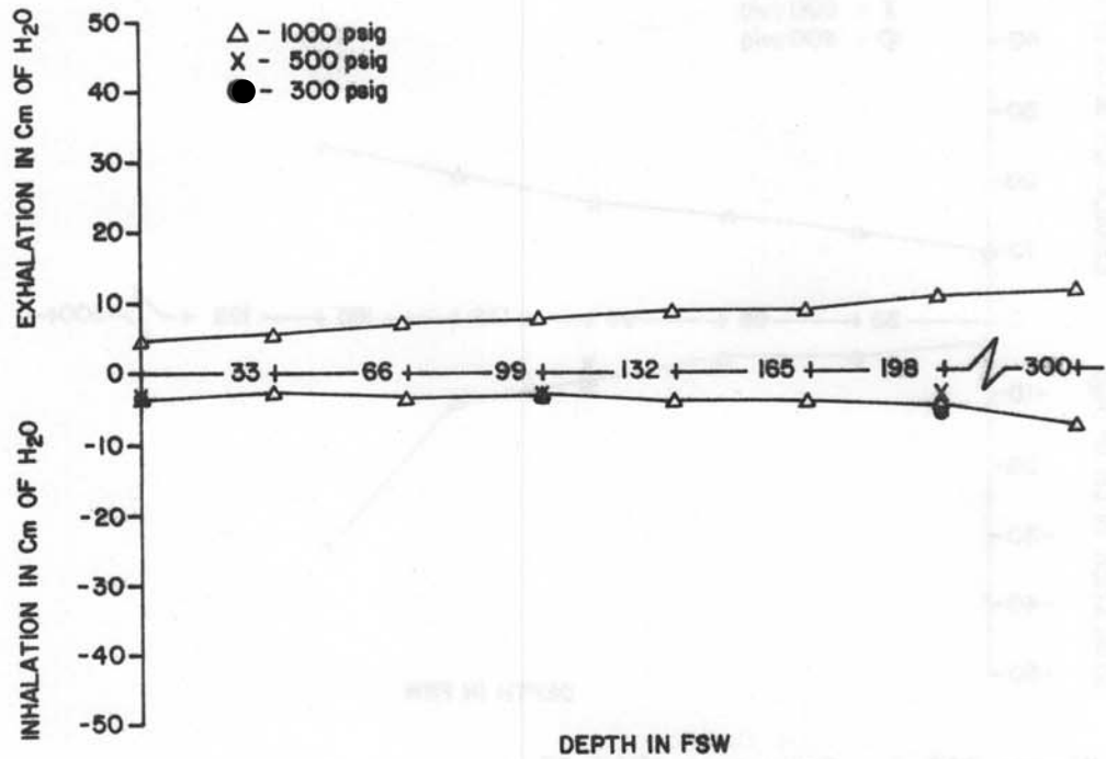
Figure 11C-1. Swimaster MR12-II Breathing resistance vs. depth at 22.5 RMV
