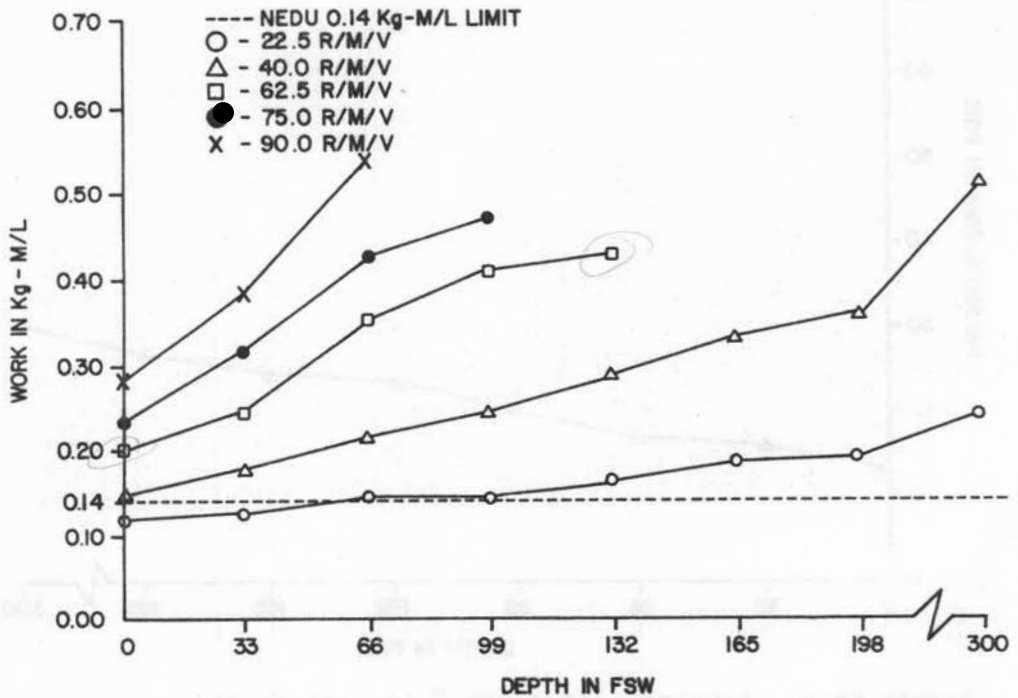
Figure 6F-6. Scubapro Air II/Mk V (4-Port Swivel) Breathing work vs. depth at 1000 psig supply pressure
