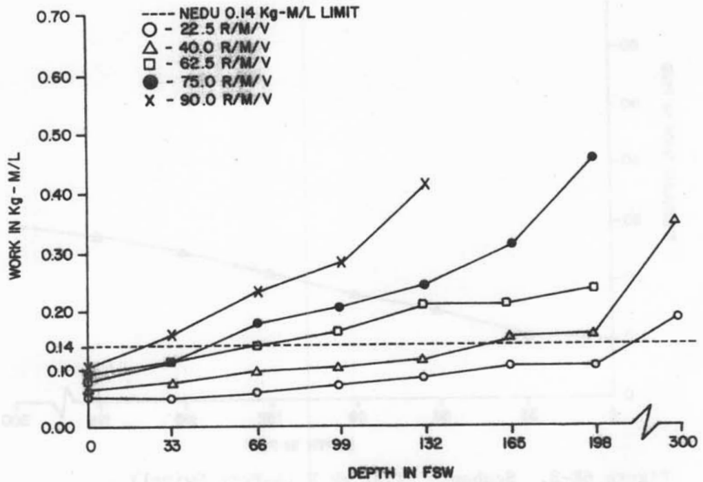
Figure 6B-6. Scubapro Pilot Mk V (4-Port Swivel) Breathing work vs. depth at 1000 psig supply pressure
