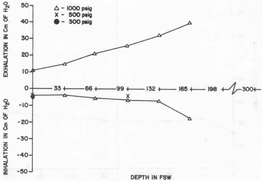
Figure 5A-5. Scubamaster Model 7687 Breathing resistance vs. depth at 90 RMV
