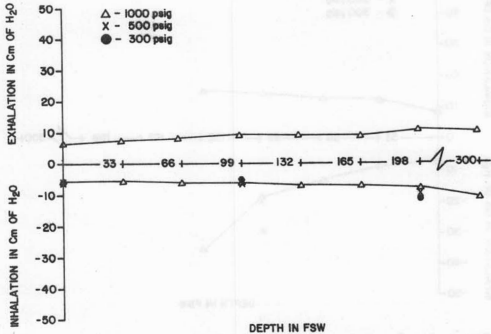
Figure 11A-1. Swimaster R14 Polaris Breathing resistance vs. depth at 22.5 RMV
