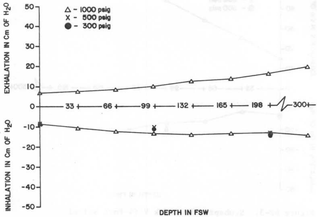
Figure 6F-1. Scubapro Air II/Mk V (4-Port Swivel) Breathing resistance vs. depth at 22.5 RMV
