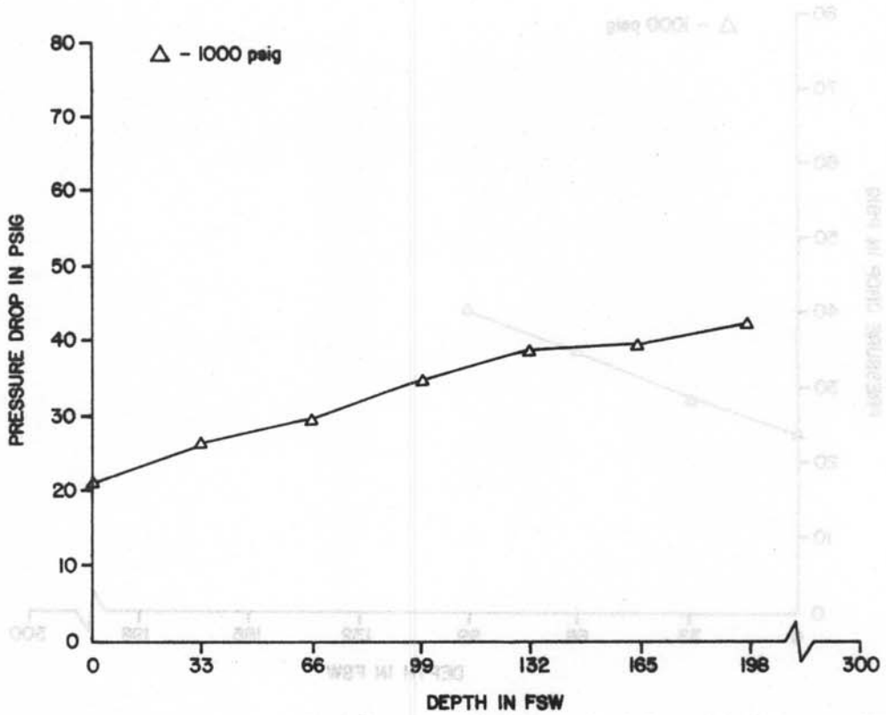
Figure 10B-9. Sub Aquatic Systems Sub X First stage pressure drop vs. depth at 62.5 RMV
