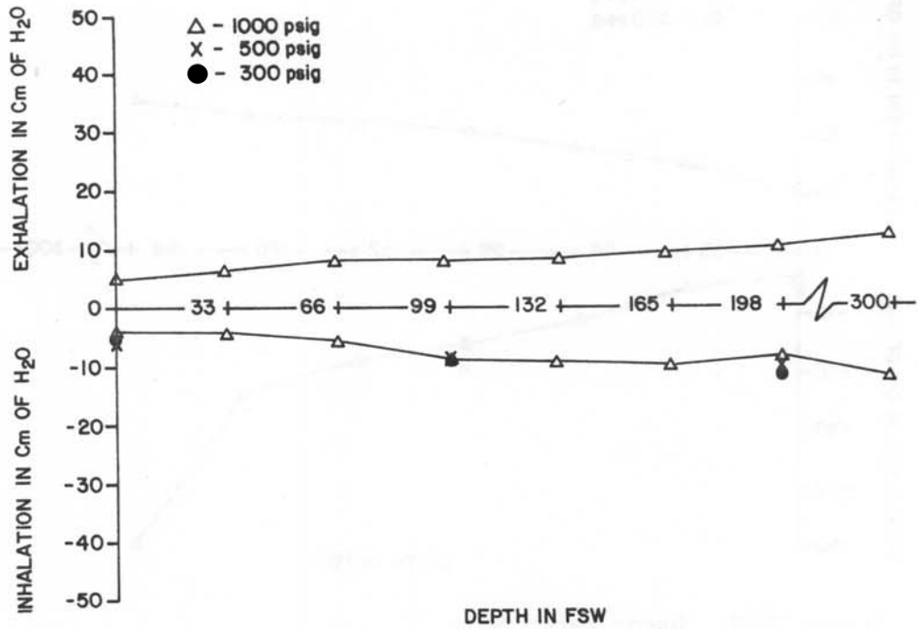
Figure 2D-1. Dacor Pacer 600 Breathing resistance vs. depth at 22.5 RMV
