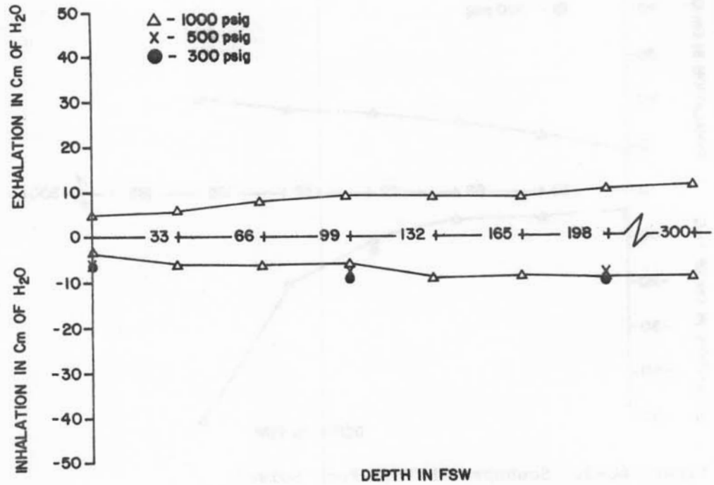
Figure 6C-1. Scubapro Mk V (5-Port Swivel) Breathing resistance vs. depth at 22.5 RMV
