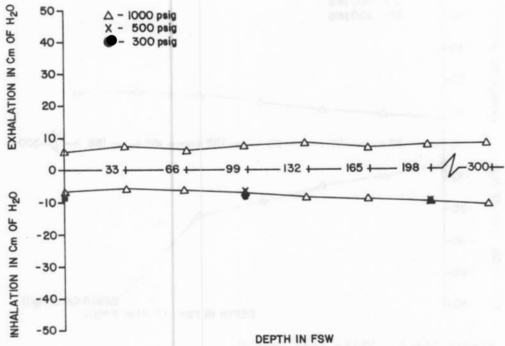
Figure 14A-1. White Stag Deep V Breathing resistance vs. depth at 22.5 RMV
