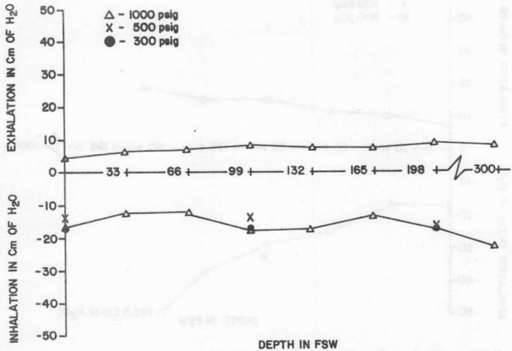
Figure 9D-1. Sportsways W-950 Arctic Breathing resistance vs. depth at 22.5 RMV
