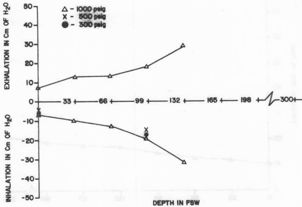
Figure 6B-5. Scubapro Pilot Mk V (4-Port Swivel) Breathing resistance vs. depth at 90 RMV
