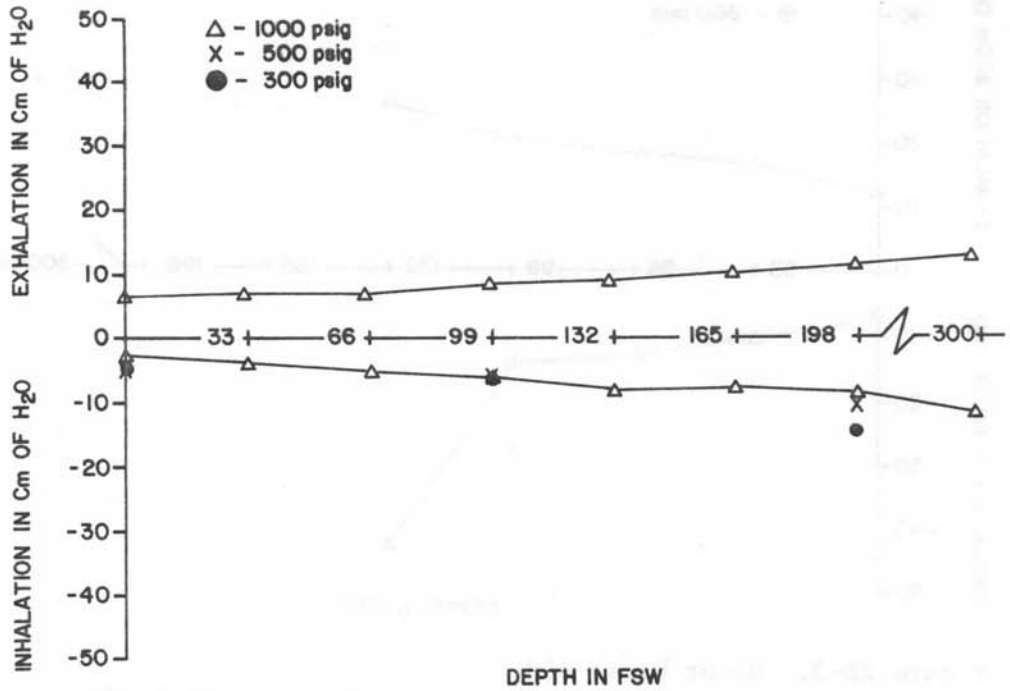
Figure 2B-1. Dacor Pacer 150 Breathing resistance vs. depth at 22.5 RMV
