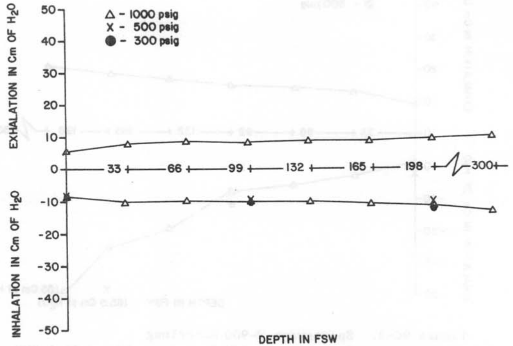
Figure 9C-1. Sportsways W-900 Waterlung Breathing resistance vs. depth at 22.5 RMV
