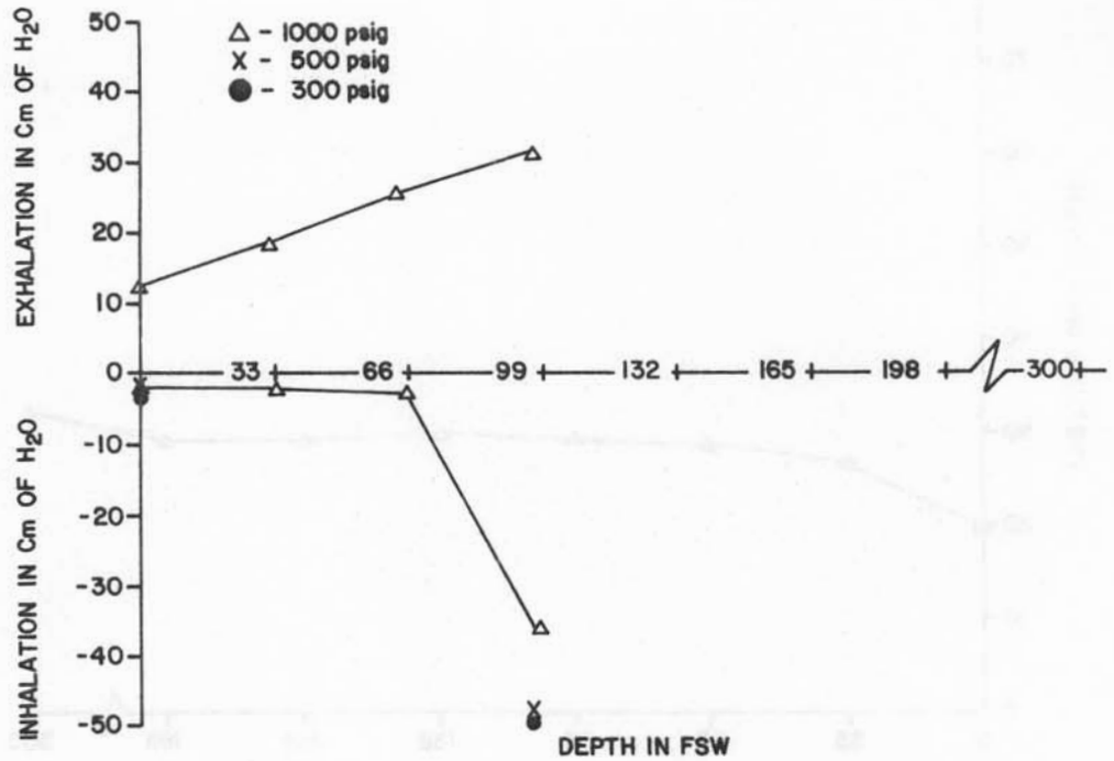
Figure 6D-5. Scubapro Air I/Mk V (4-Port Swivel) Breathing resistance vs. depth at 90 RMV
