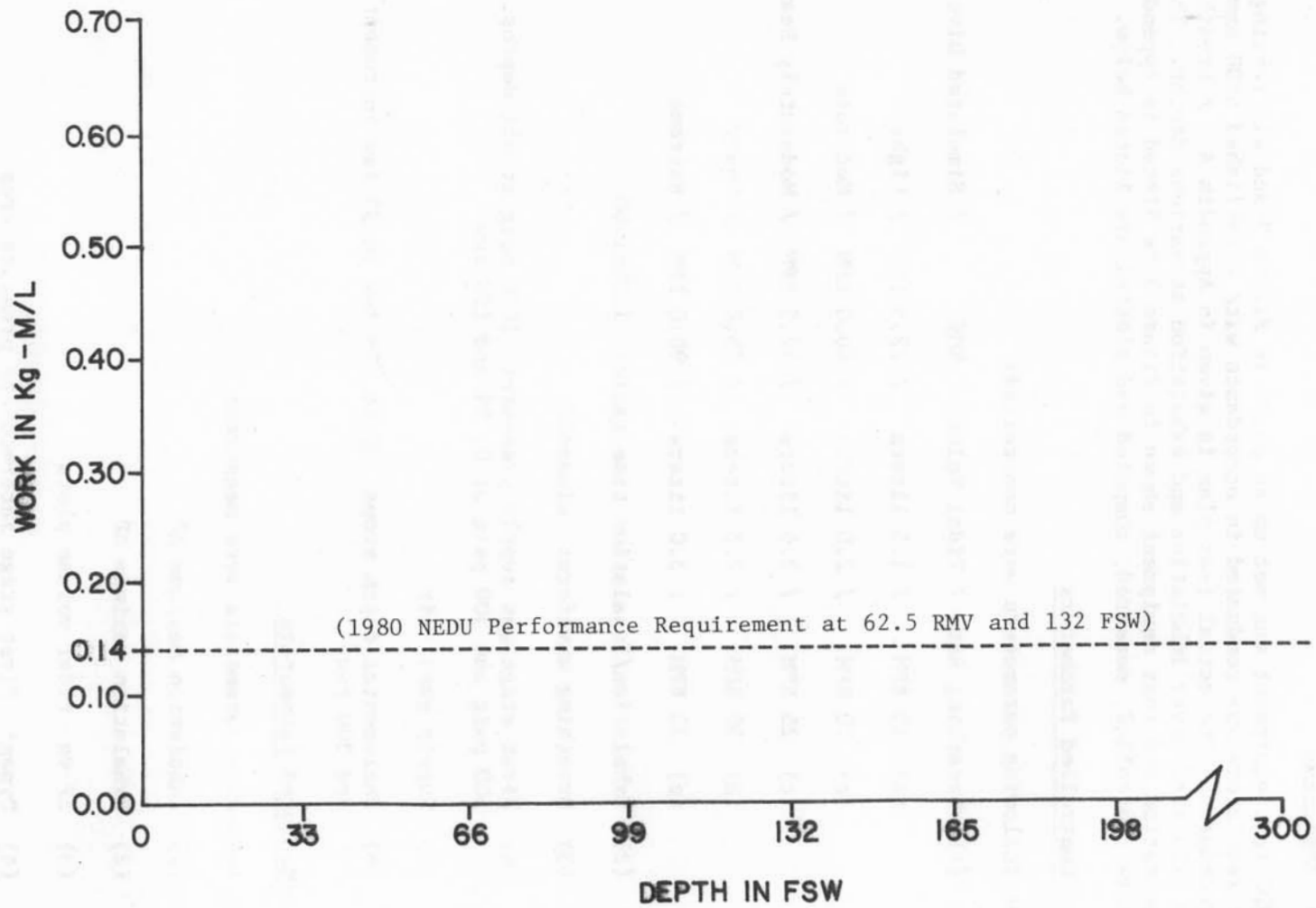
Figure 2. 1980 NEDU scuba regulator performance requirement
