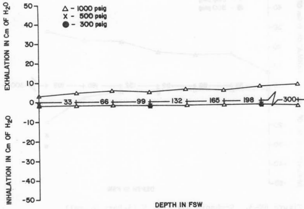
Figure 6E-1. Scubapro Air I/Mk V (5-Port Swivel) Breathing resistance vs. depth at 22.5 RMV
