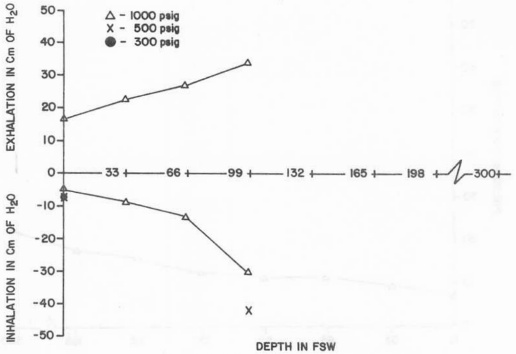
Figure 2E-5. Dacor Pacer 900 Breathing resistance vs. depth at 90 RMV
