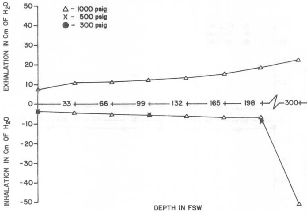
Figure 13C-3. U. S. Divers Conshelf XIV Breathing resistance vs. depth at 62.5 RMV
