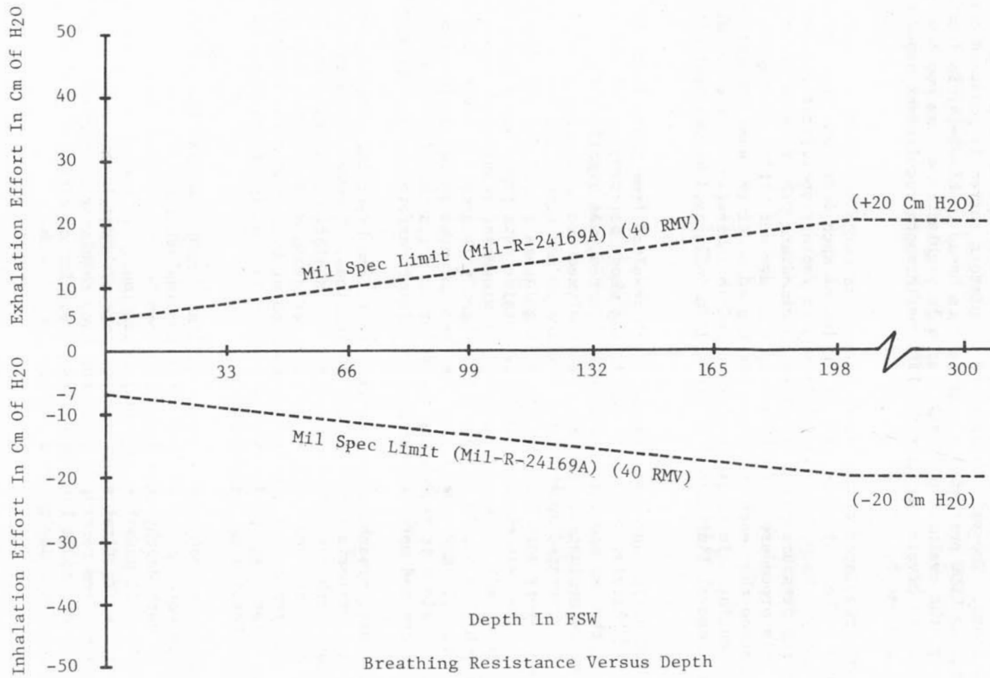
Figure 1. Previous NEDU scuba regulator performance requirement at 40 RMV
