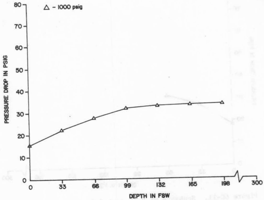
Figure 6C-9. Scubapro Mk V (5-Port Swivel) First stage pressure drop vs. depth at 62.5 RMV
