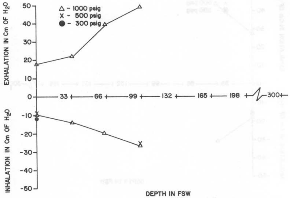
Figure 2A-3. Dacor C3NB Breathing resistance vs. depth at 62.5 RMV
