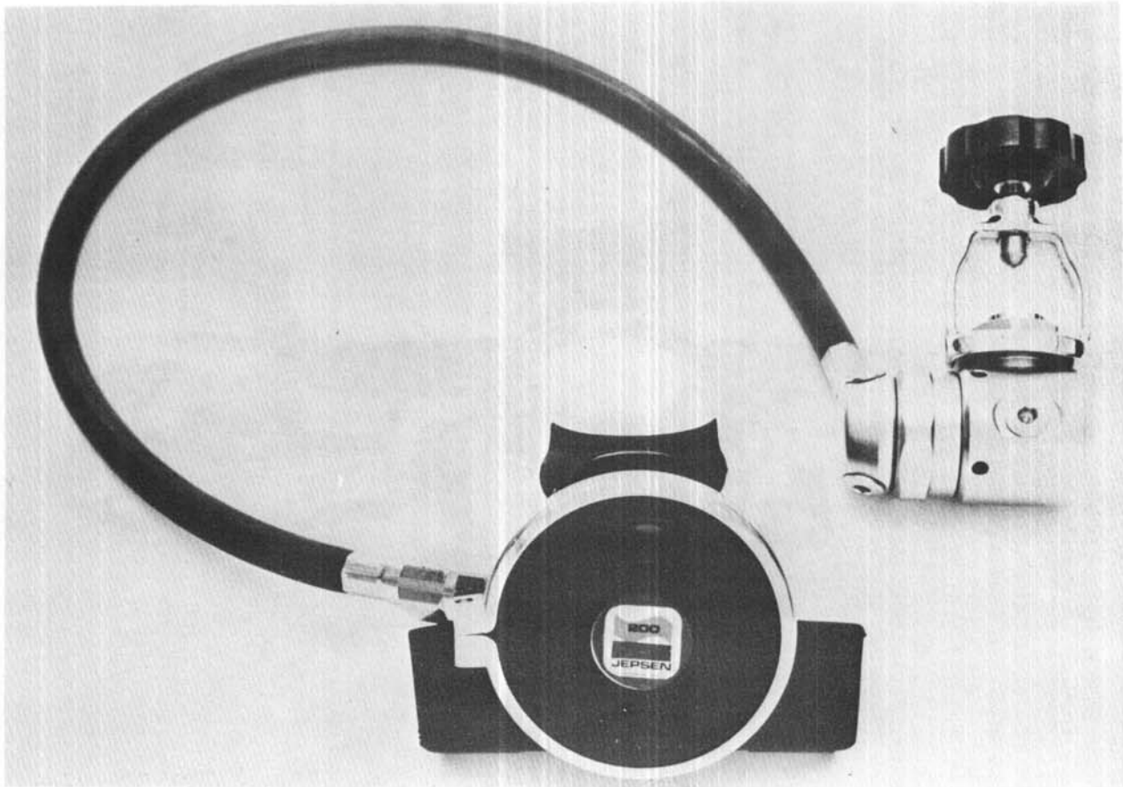
Jepsen Model 200
