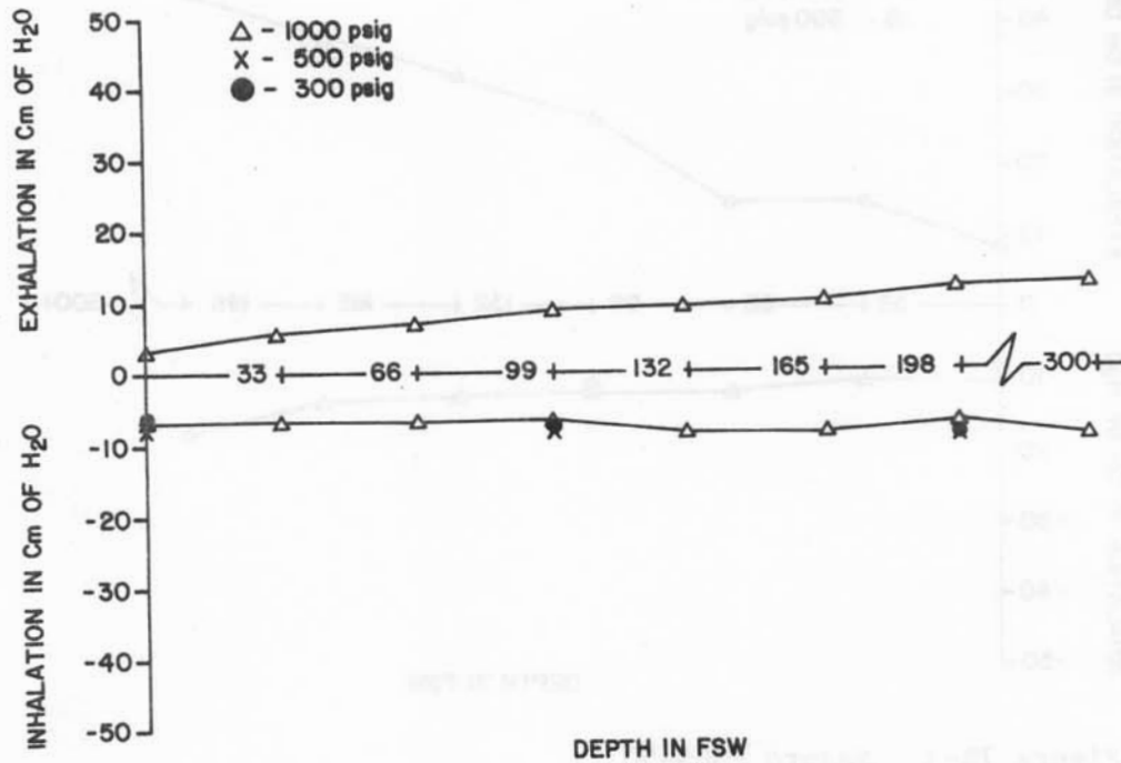
Figure 7B-1. Seapro FSDS-50 Breathing resistance vs. depth at 22.5 RMV
