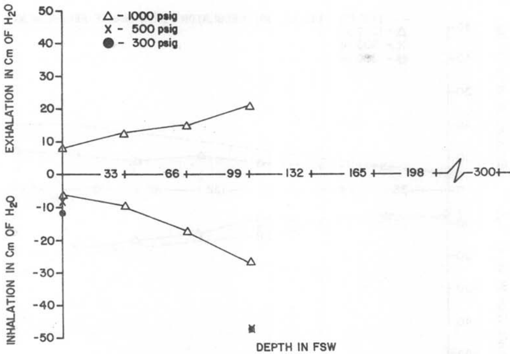
Figure 14A-4. White Stag Deep V Breathing resistance vs. depth at 75 RMV
