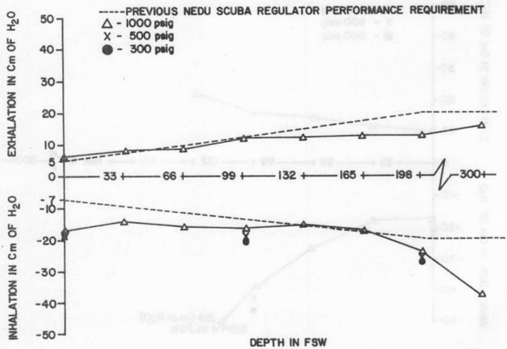
Figure 9D-2. Sportsways W-950 Arctic Breathing resistance vs. depth at 40 RMV
