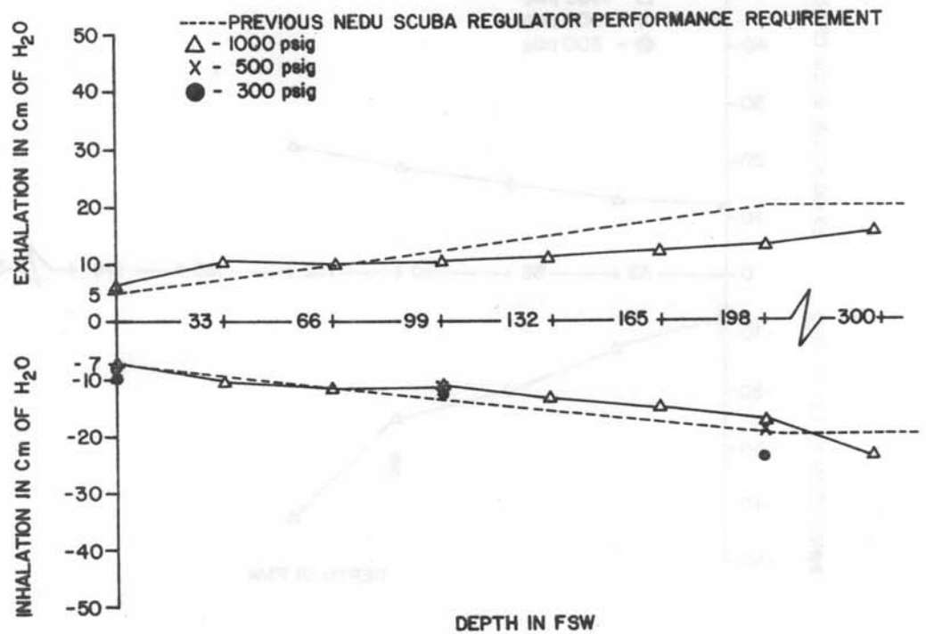
Figure 9C-2. Sportsways W-900 Waterlung Breathing resistance vs. depth at 40 RMV
