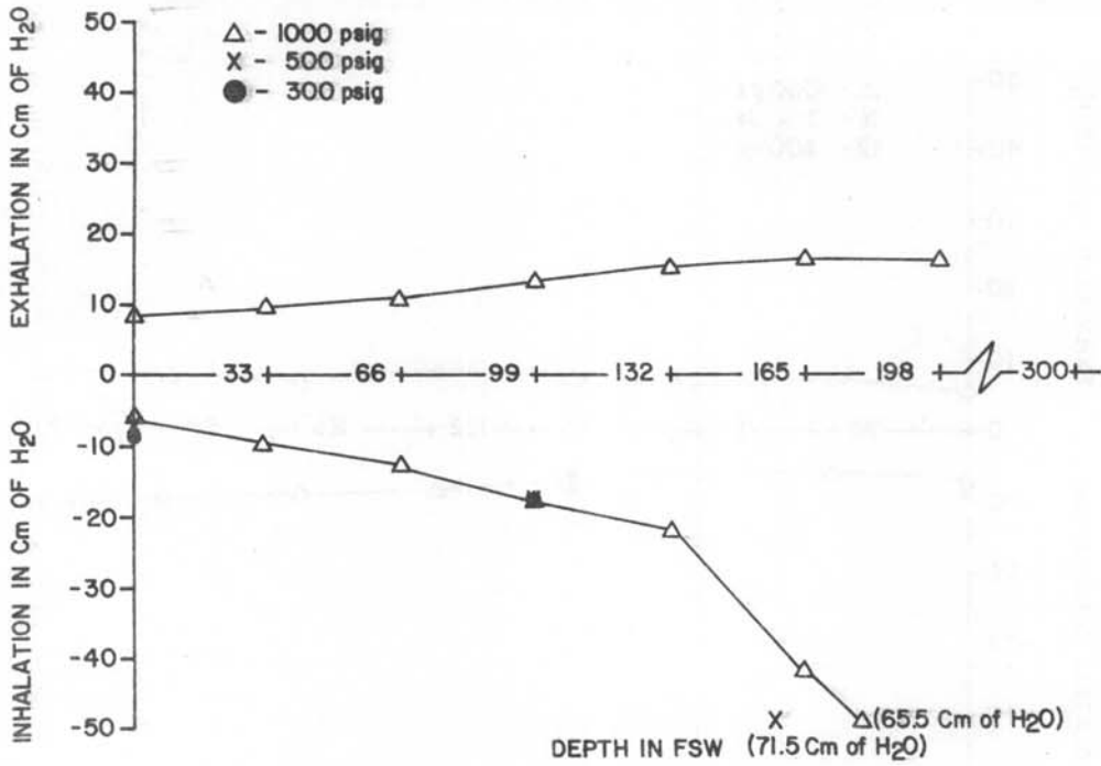
Figure 14A-3. White Stag Deep V Breathing resistance vs. depth at 62.5 RMV
