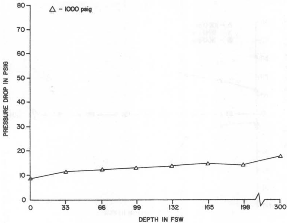
Figure 11C-7. Swimmaster MR12-II First stage pressure drop vs. depth at 22.5 RMV
