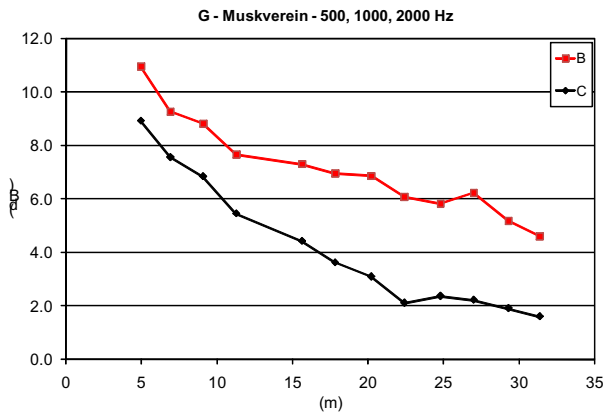
Fig 11 Strength at mid frequencies G
