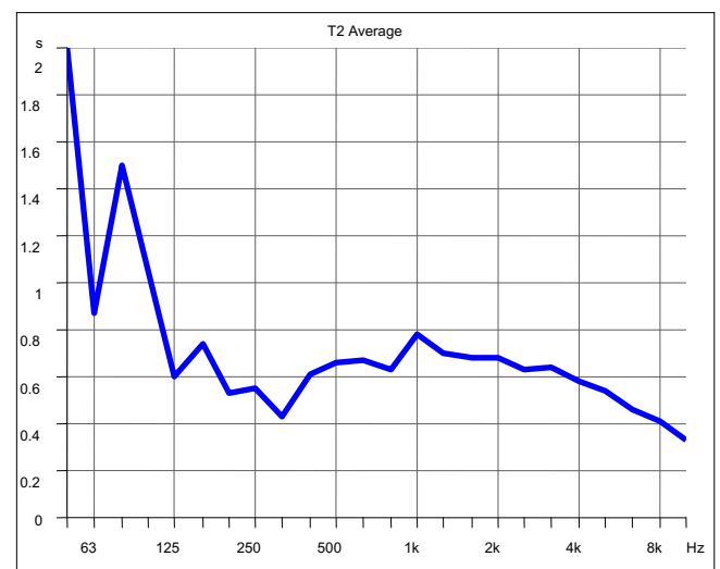
Fig 14 Reverberation Time T30 – Storage Room
