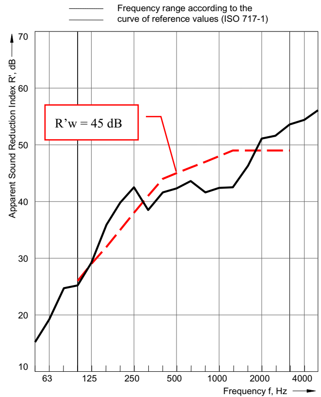
Fig 13 Sound Reduction Index
