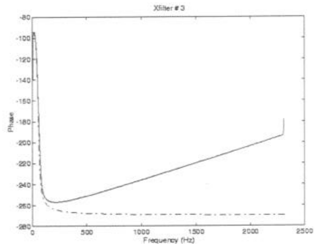
Fig. 6. Phase of H_x filter from Small-Thiele model. (ideal: dashed line ; FIR implemented on DSP: solid line)
