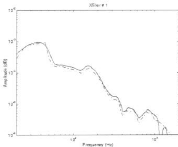
Fig. 7. Magnitude of H_x filter from SPL measurements. (ideal: dashed line ; FIR implemented on DSP: solid line)
