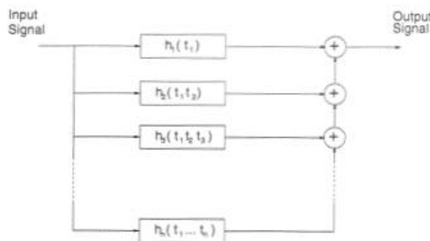
Fig. 1. Block diagram of Volterra series expansion.
