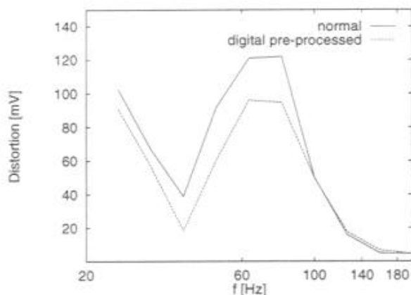
Fig. 14. Comparison between the THD of the considered loudspeaker with and without the audio processor (3 Volt input signal amplitude).
