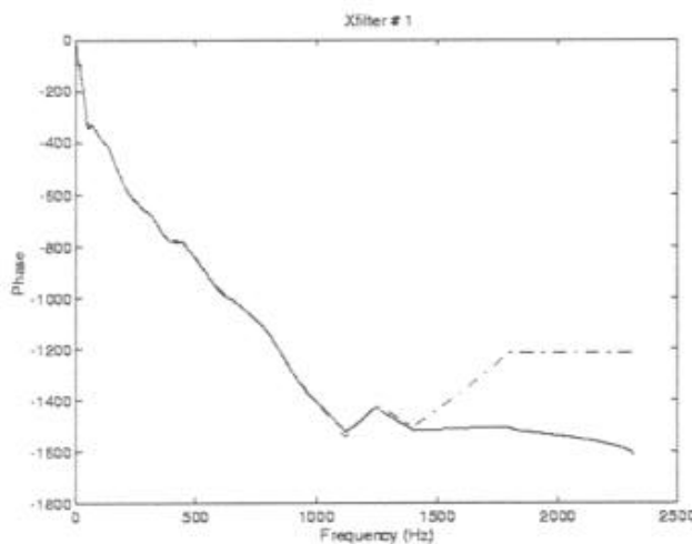
Fig. 8. Phase of H_x filter from SPL measurements. (ideal: dashed line ; FIR implemented on DSP: solid line)
