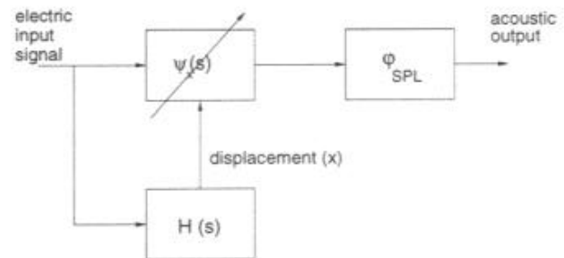
Fig. 4. Block diagram of the second loudspeaker model.
