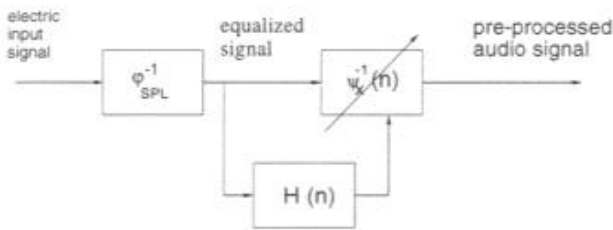
Fig. 10. Block diagram of the inverse filter.
