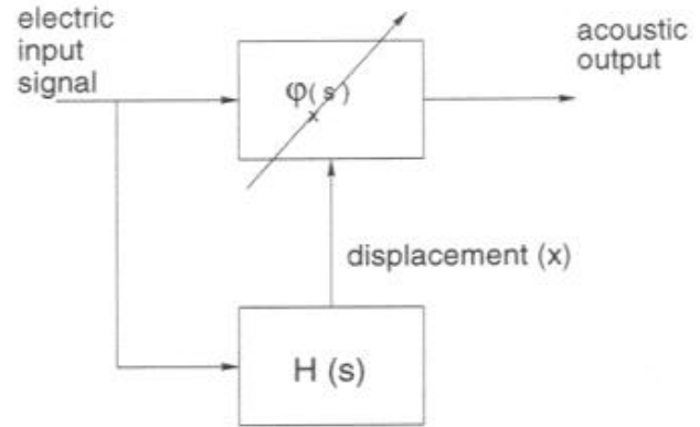
Fig. 3. Block diagram of the first loudspeaker model.
